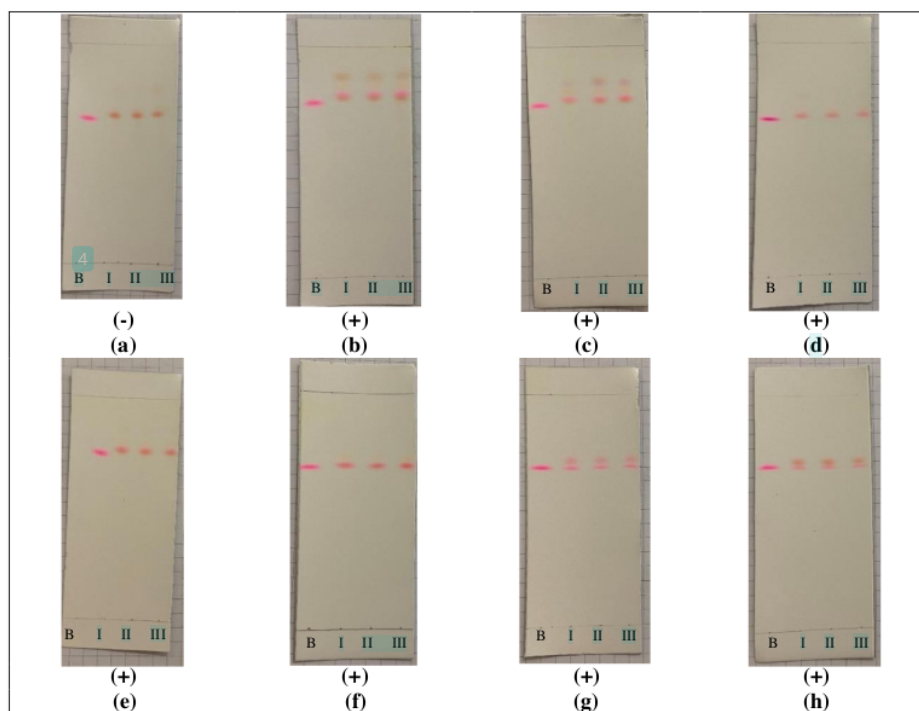
Figure 2. Visually spot sample
