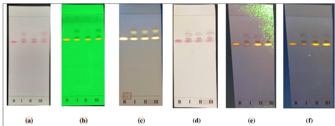
Figure 1. Spots of mobile phase n-Butanol : Ethanol : Aquadest (20:12:15)
