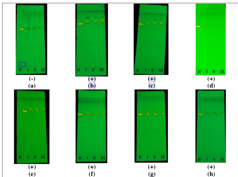
Figure 3. Sample spot under 254 nm UV light
