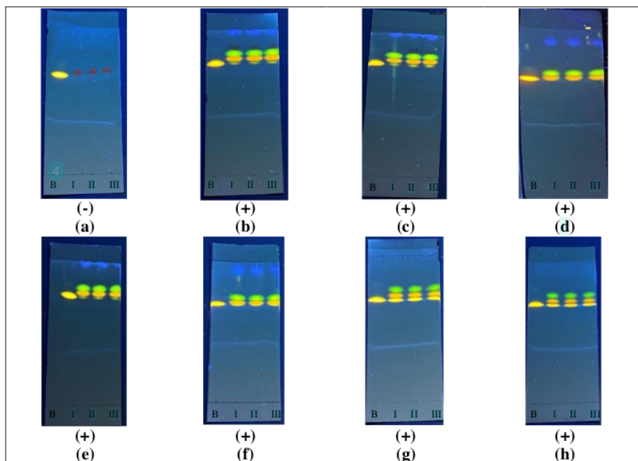
Figure 4. Sample spot under 366 nm UV light
