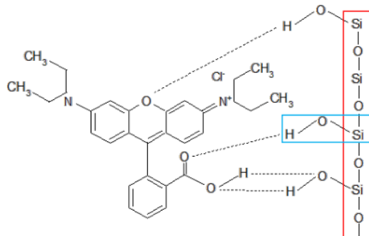
Figure 6. Rhodamine B . Hydrogen Bond Interaction
